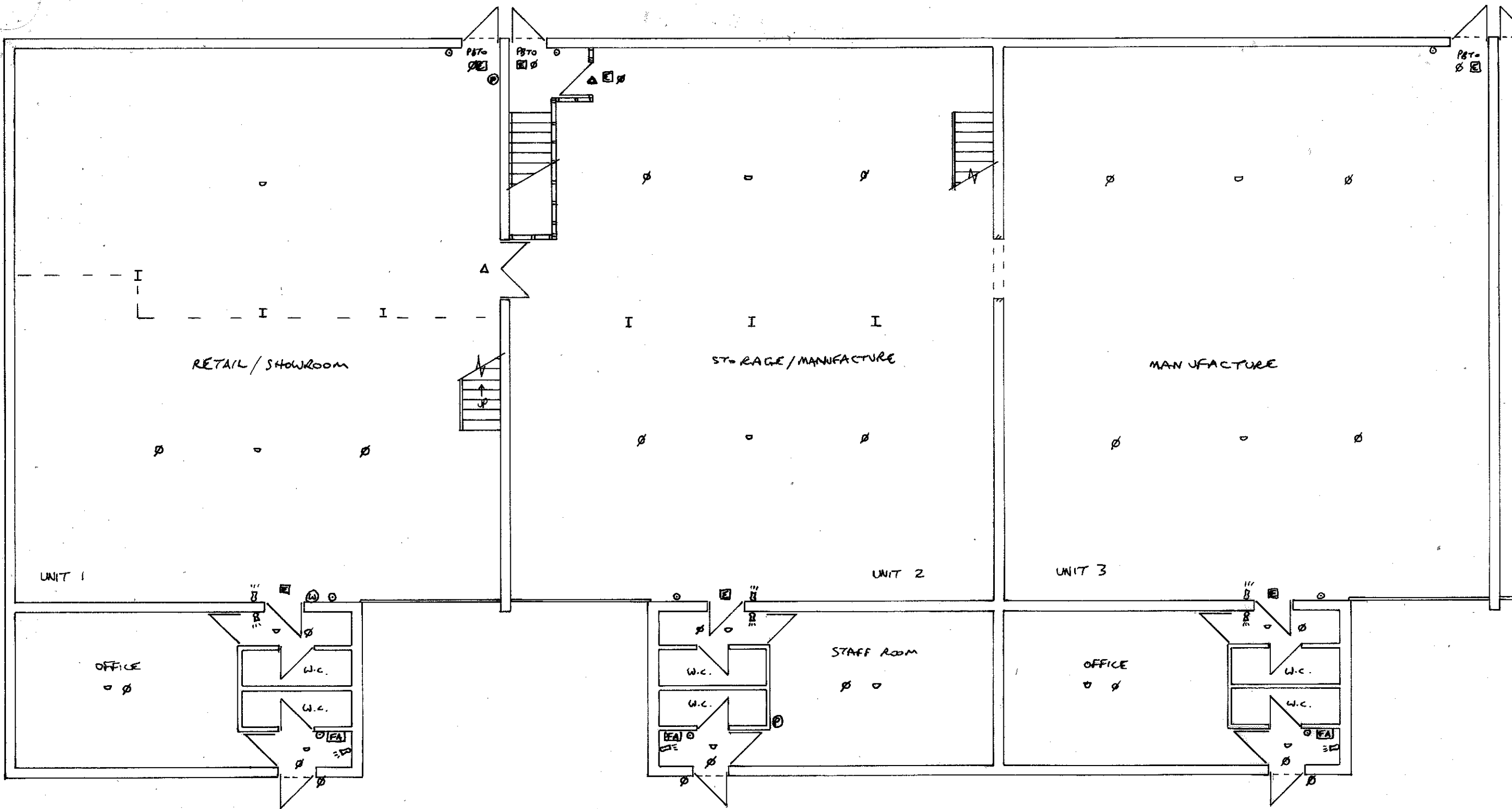
PROPOSED GROUND FLOOR 1:100
